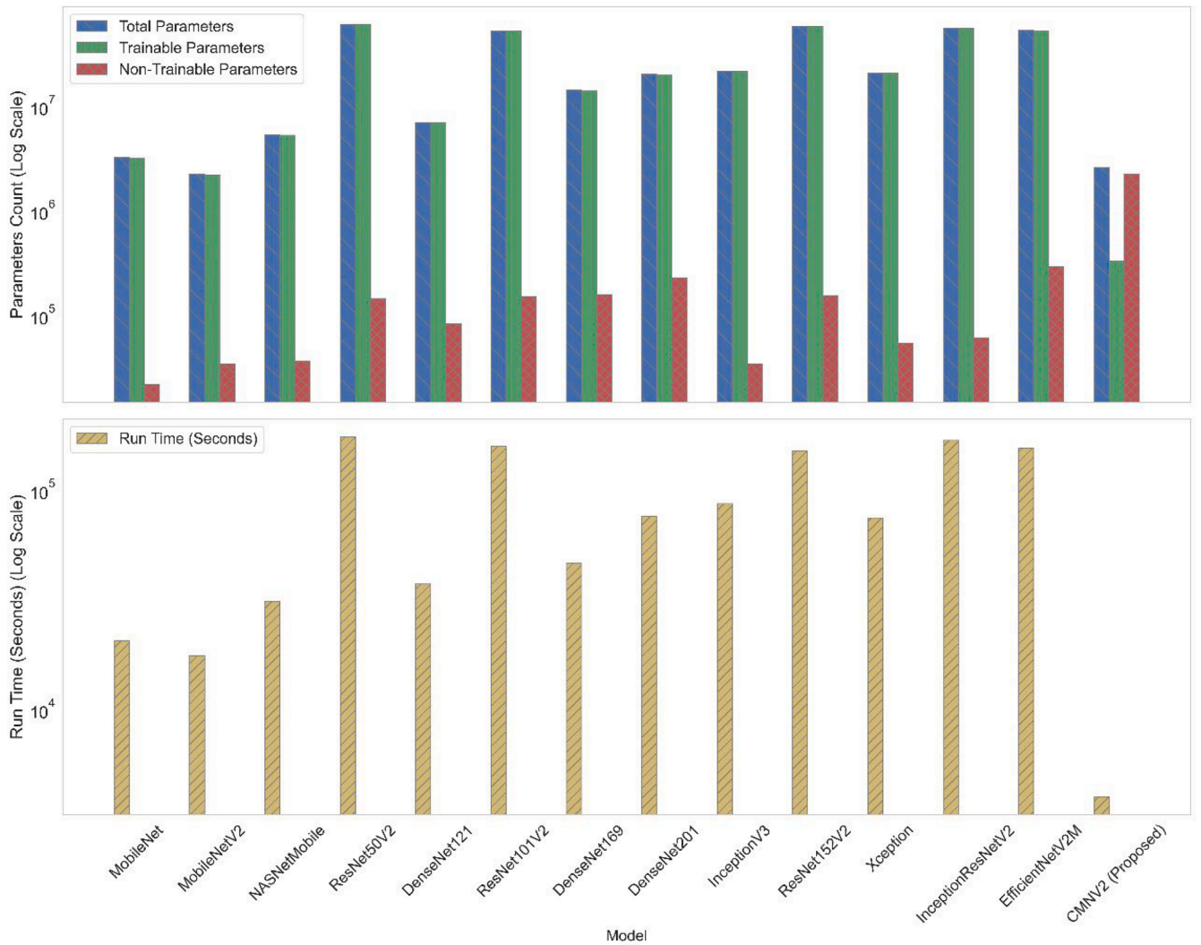
Fig. 6. Log-scaled comparison of model complexity and execution time of 14 models.
