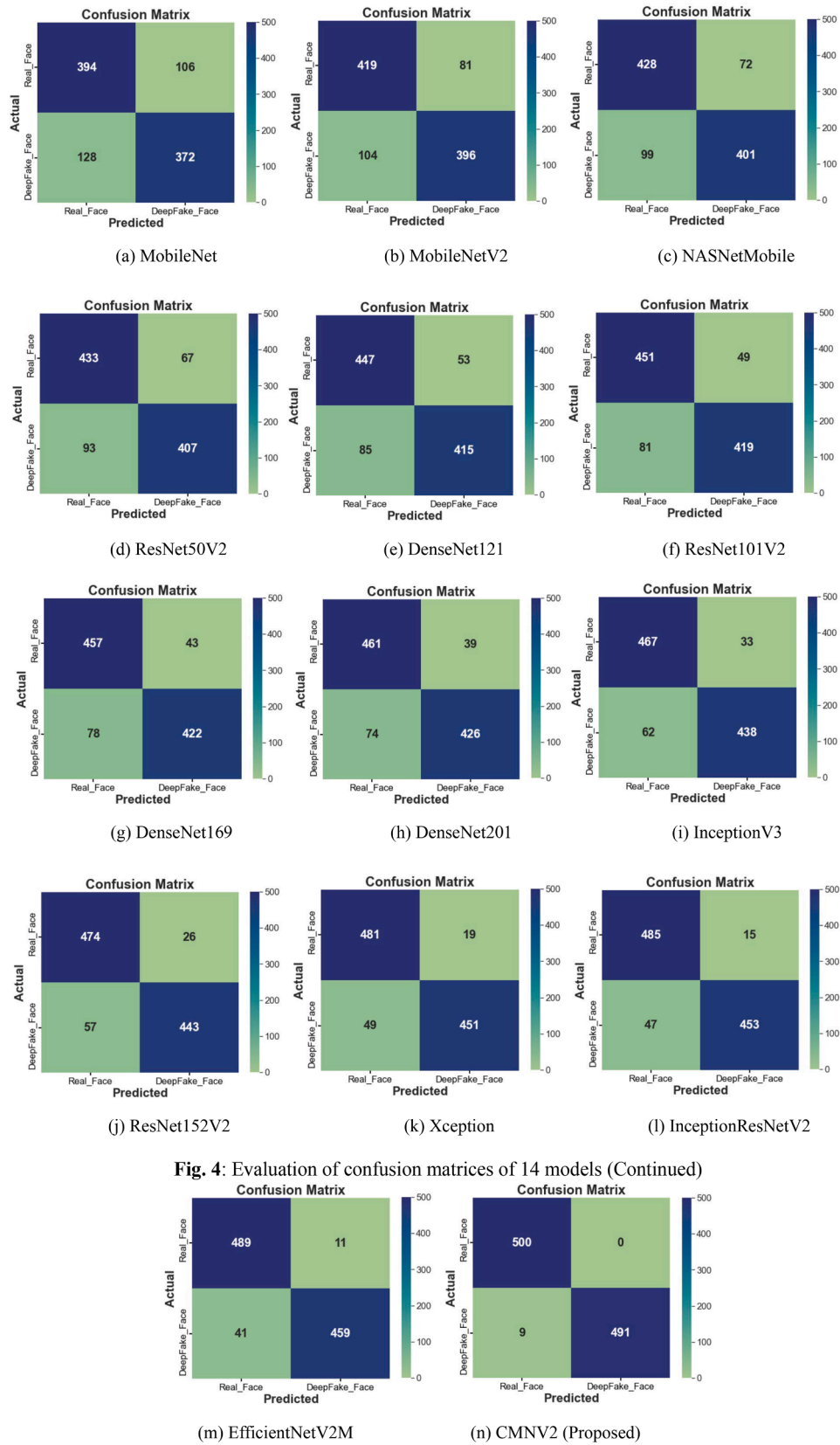
Fig. 4: Evaluation of confusion matrices of 14 models (Continued) Fig. 4: Evaluation of confusion matrices of 14 models.
