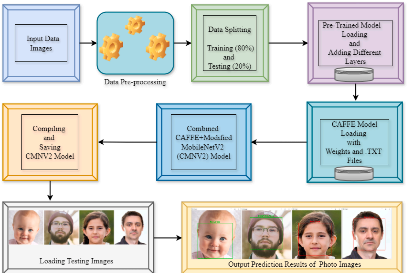
Fig. 3. CMNV2 block diagram.
