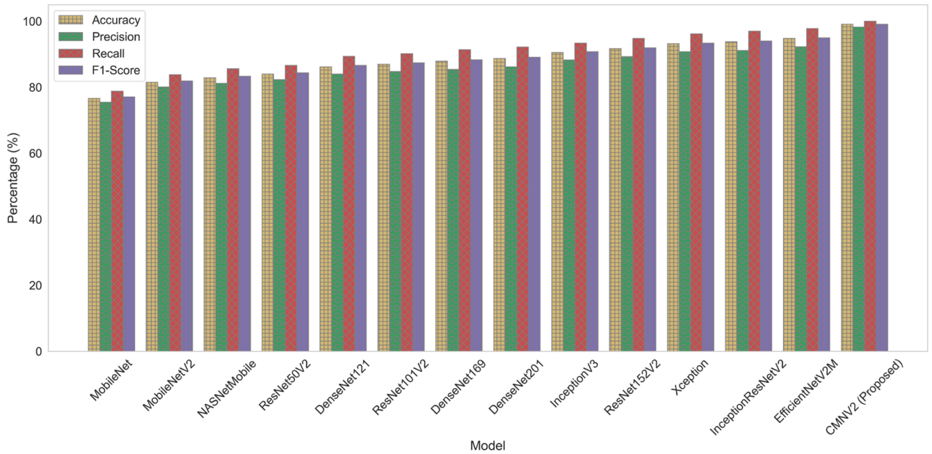
Fig. 5. All 14 models statistical performance analysis.
