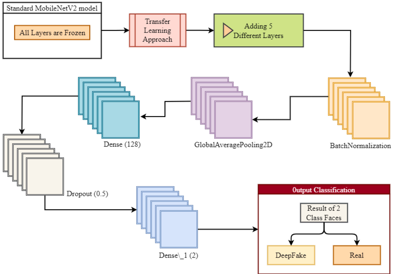
Fig. 2. Customized MobileNetV2 framework.
